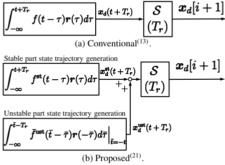
Fig. 3. State trajectory generation.
