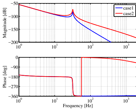
Fig. 6. Bode diagram of P_c(s) .
